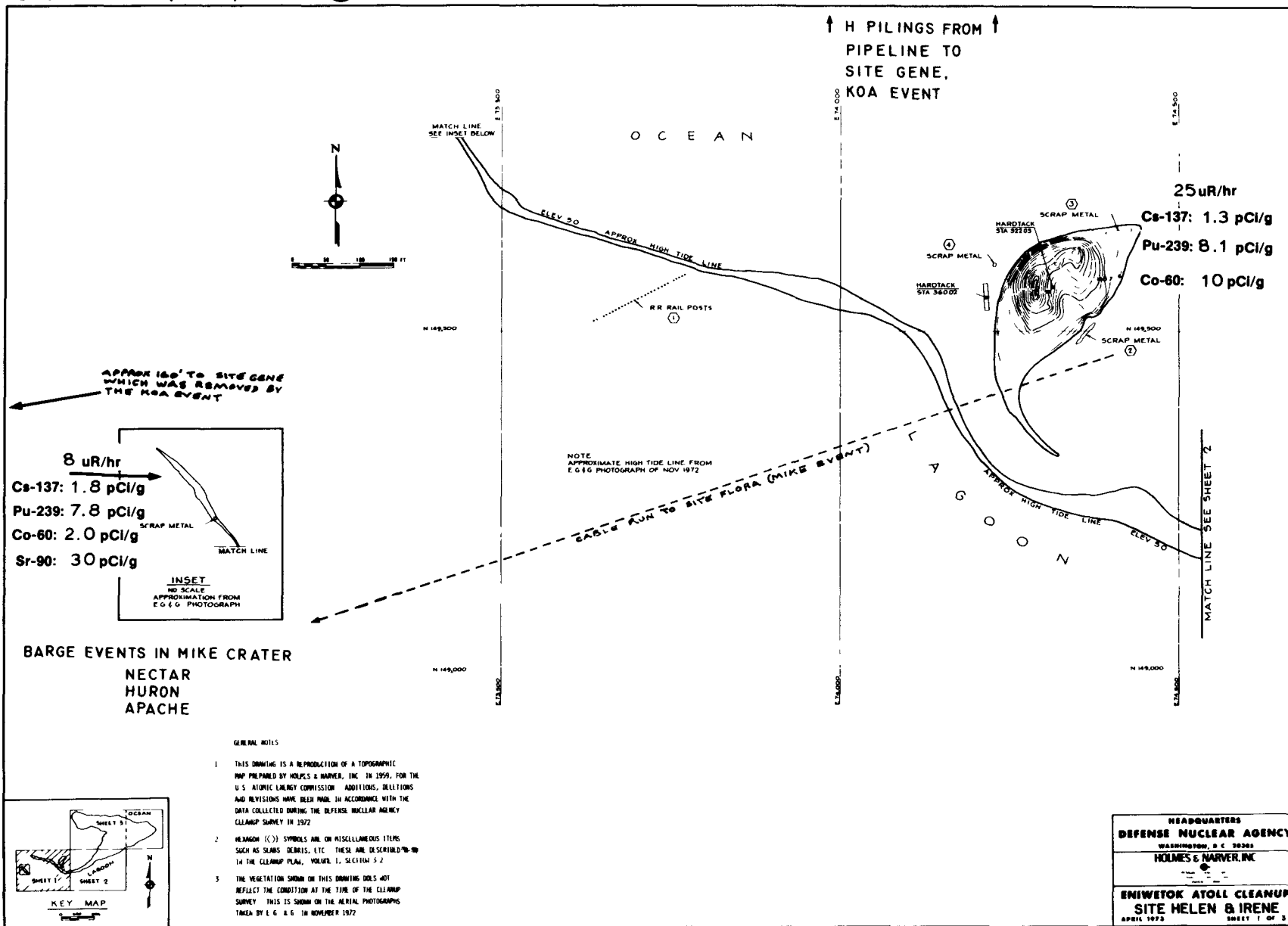
FIGURE 8. SITES HELEN AND IRENE, SHEET 1 OF 3
